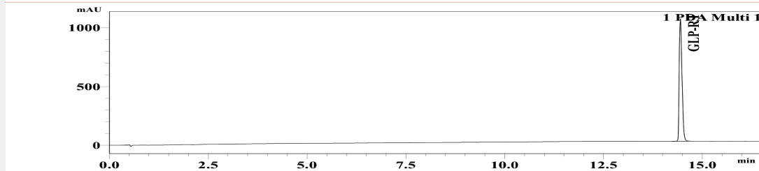
Mass Confirmation
